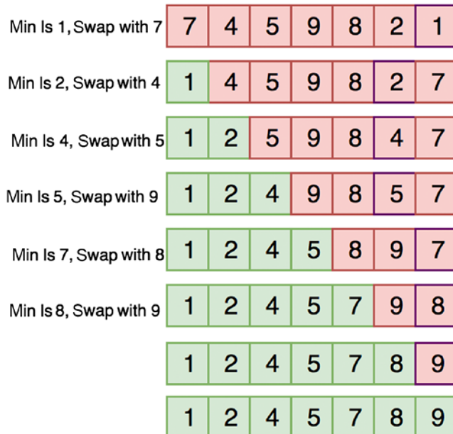
Figure 10-6. Selection sort
