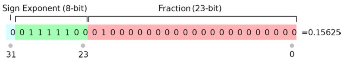
Figure 3-1. The 32-bit floating-point number system
